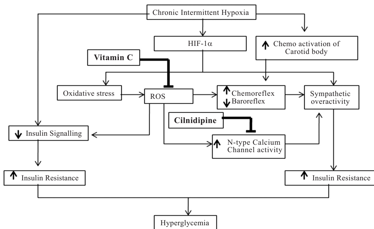
Fig. (5). Schematic diagram outlining the hypothesized pathways by which chronic intermittent hypoxia leads to hyperglycemia.
