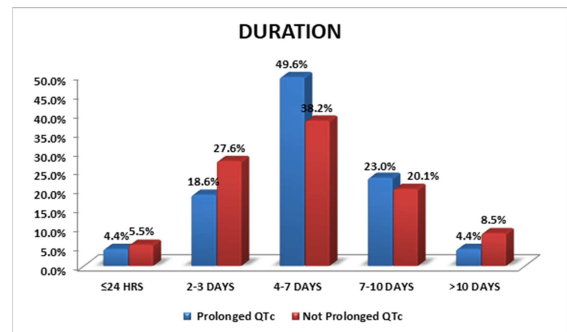
Figure 4: distribution of duration according to QTc
