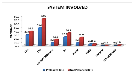
Figure 3: distribution of system involved according to QTc
