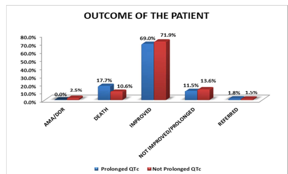
Figure 5: Distribution of Outcome According to QTc
