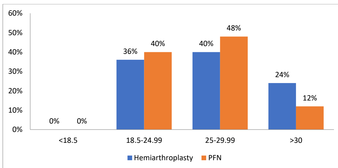
Figure 4: Comparison of groups according to BMI
