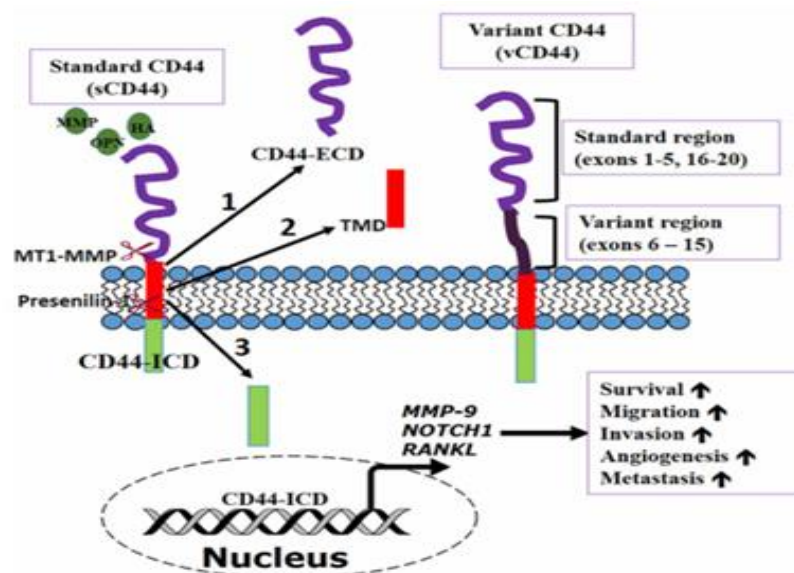
Figure 4: CD44, a multifunctional receptor, plays a crucial role in regulating biological processes related to cancer cell spreading and metastasis. CD44 can be successively cleaved by membrane type 1 matrix metalloproteinase (MT1-MMP) and subsequently by presenilin-1/ \gamma -secretase, which is activated by the
